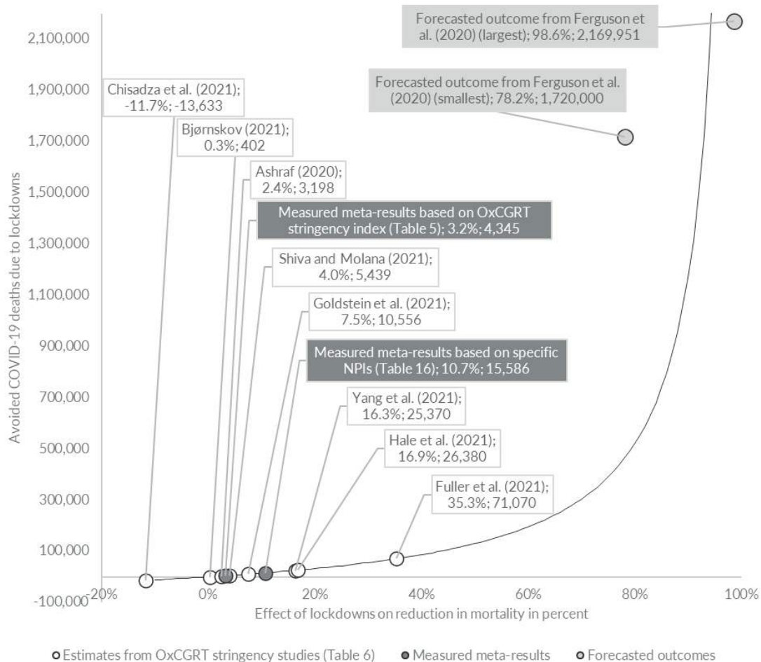
Figure 10: Divergence between avoided number of deaths in the United States as measured by the meta-results, studies based on the OxCGR stringency index, and the forecasted outcome from Imperial College London
