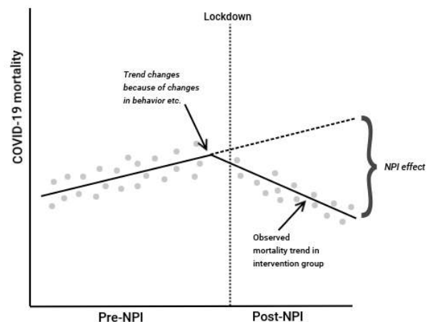
Figure 5: Simplified illustration of the difference-in-difference approach compared to interrupted time series approach when trends changes
